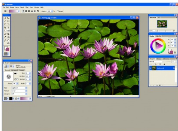
Artweaver
